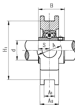
UCT2 带顶丝
