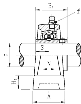
UCP200M 带顶丝
