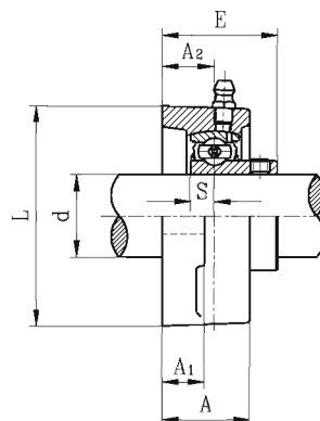
SBFL2G 带顶丝
