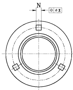
PF
