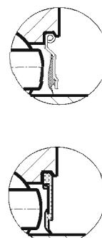
RS密封 (+后缀-2RS)
