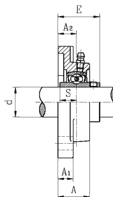
UCFX 带顶丝
