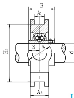
UCT3 带顶丝
