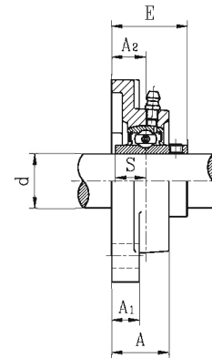
UCF3 带顶丝
