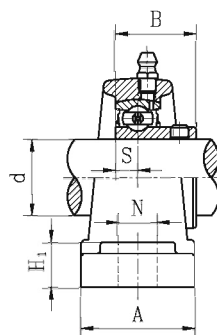
SBP2G 带顶丝
