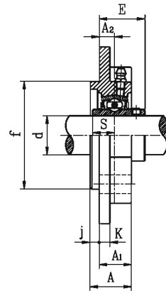
UCFC2 带顶丝
