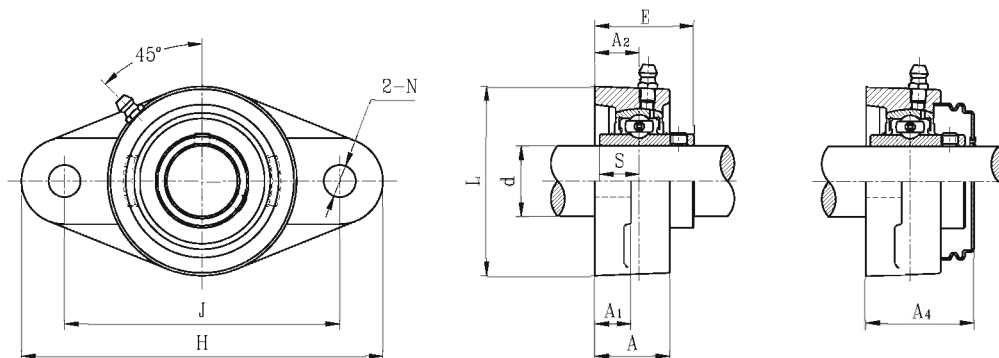
UCFL2 带顶丝
