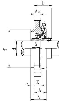
UCFS3 带顶丝
