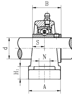
UCP2 带顶丝
