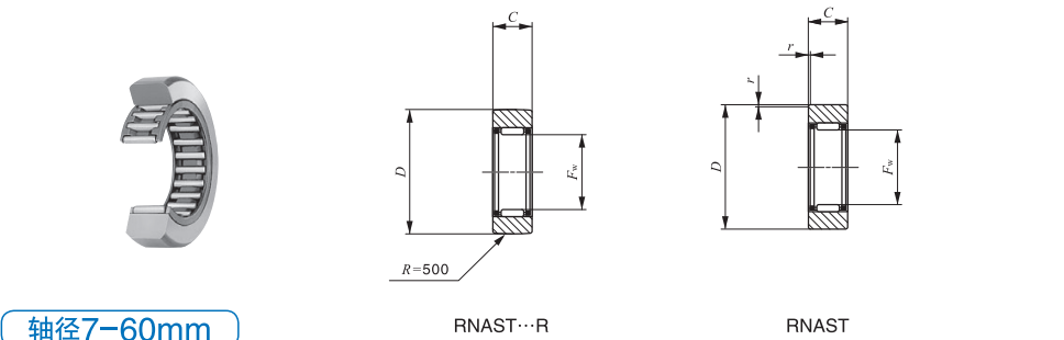
轴径7-60mm
