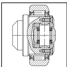
ADJUSTABLE COMBINED BEARINGS GALETS COMBINES RÉGLABLES
