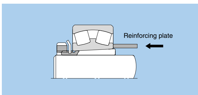
Fig. 15.21 Disassembly of bearing with adapter
