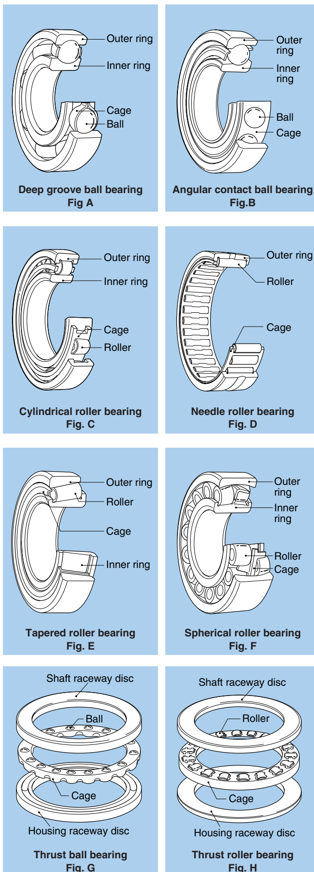
Fig. 1.1 Rolling bearing
