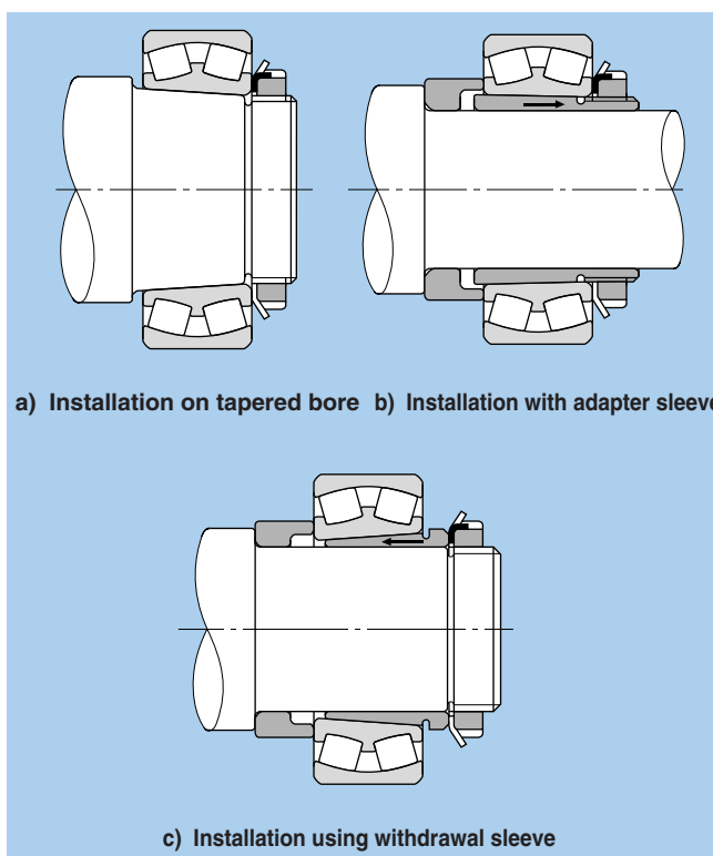
Fig. 15.7 Installation methods using locknuts
