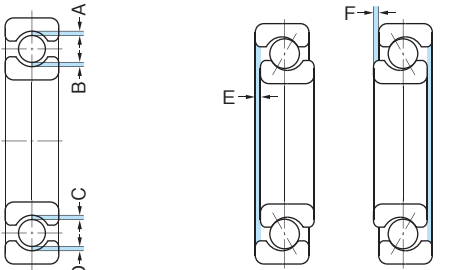
图6.1 径向游隙 =A+B+C+D
