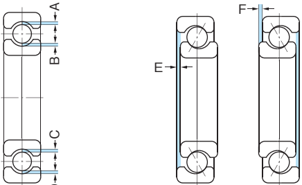
图6.1 径向游隙 =A+B+C+D
