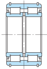
橡胶密封圈(E50...NRNT) 带止动环
